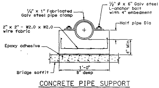
CONCRETE PIPE SUPPORT
