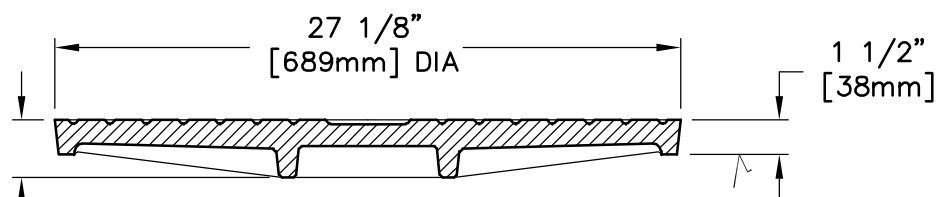
COVER SECTION
