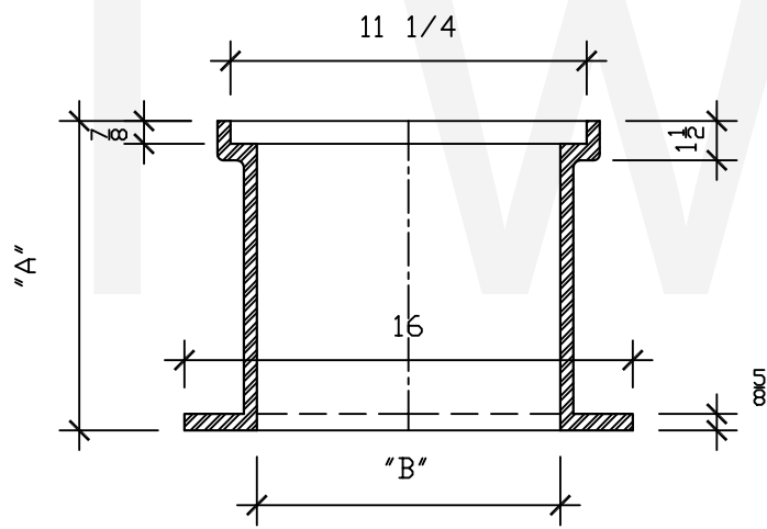
SECTION B-B ACCESS FRAME
