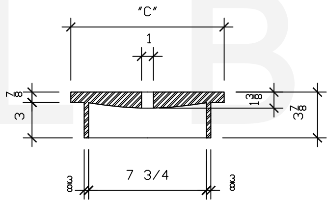
SECTION A-A ACCESS COVER
