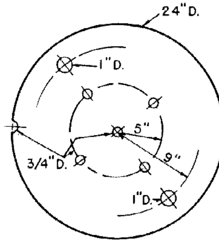
DETAIL OF HOLES IN COVER
