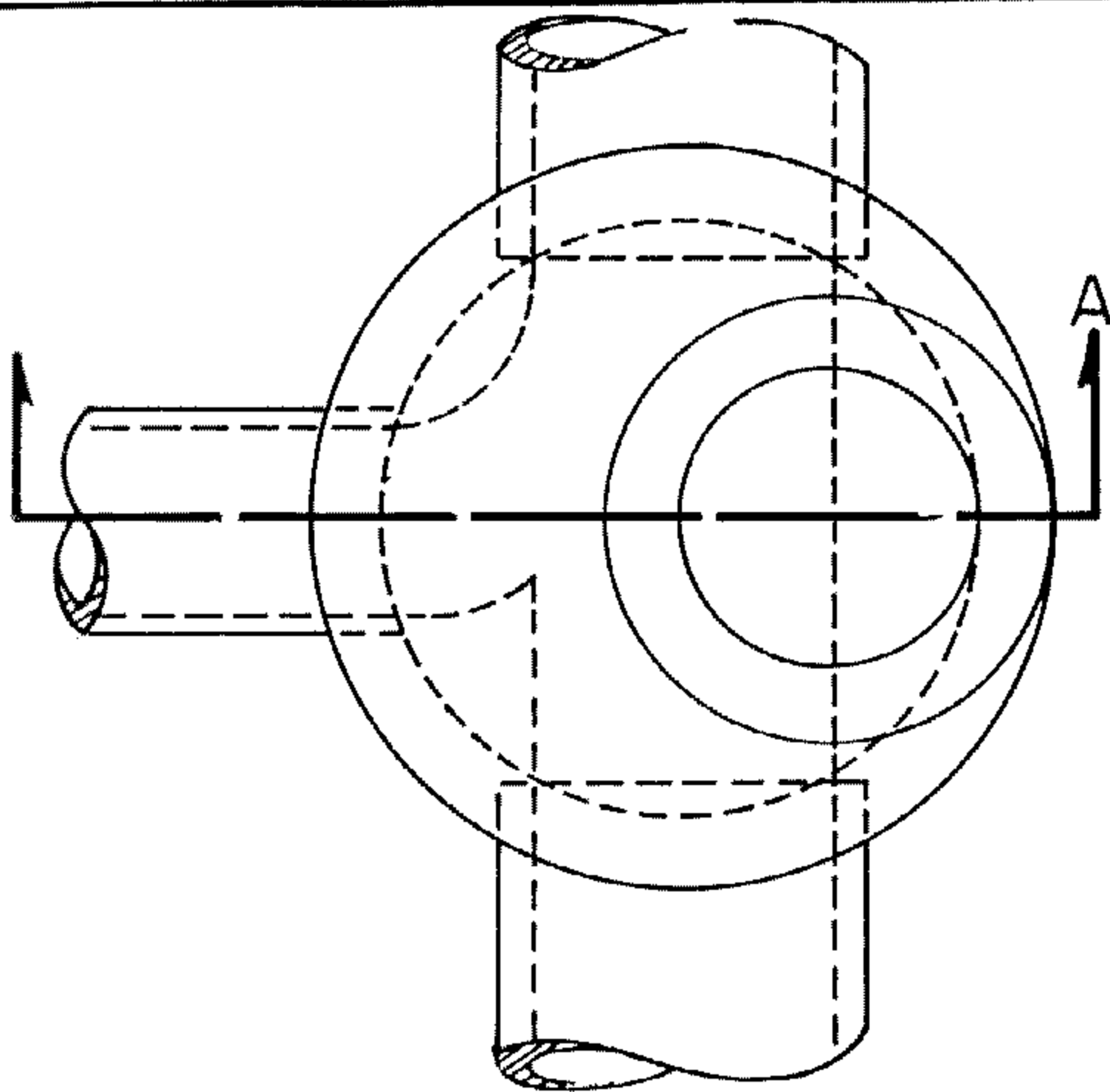
PLAN VIEW
