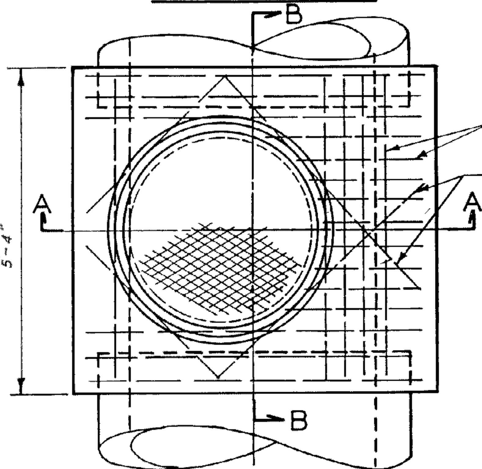
PLAN VIEW
