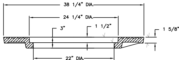
OUTER COVER SECTION
