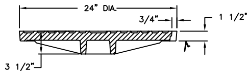
INNER COVER SECTION
