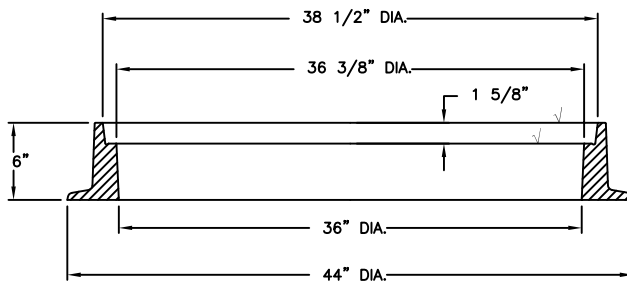
FRAME SECTION
