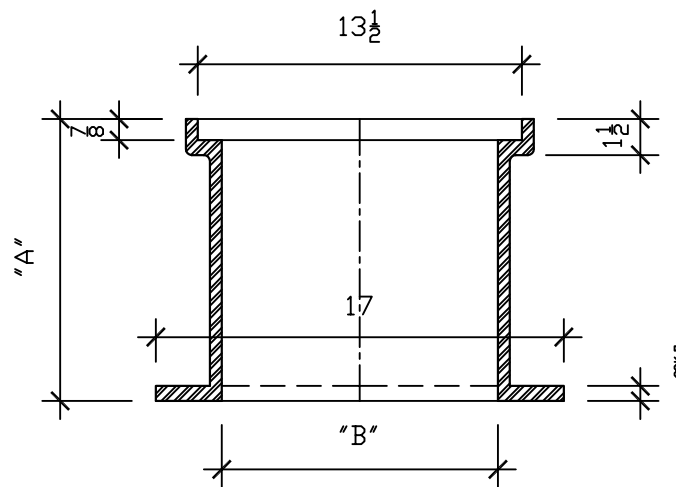
ACCESS FRAME
