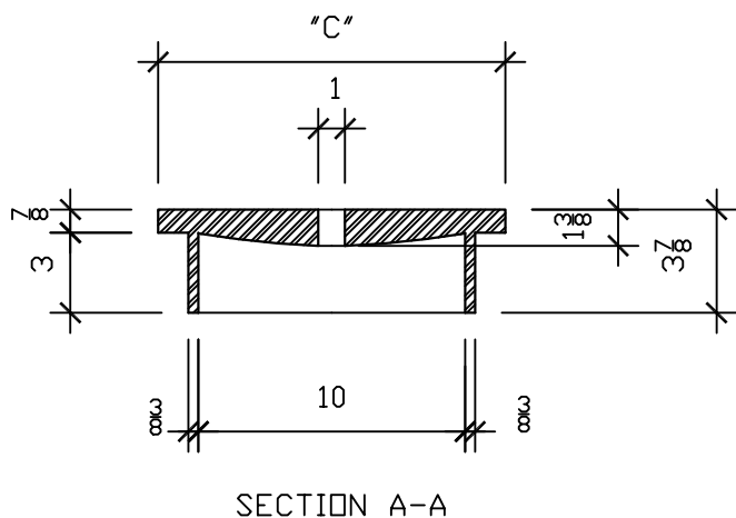
ACCESS COVER
