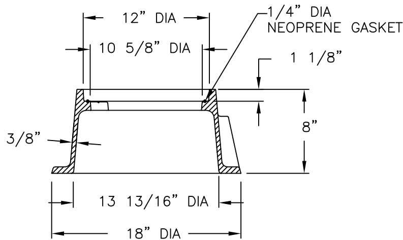
FRAME SECTION
