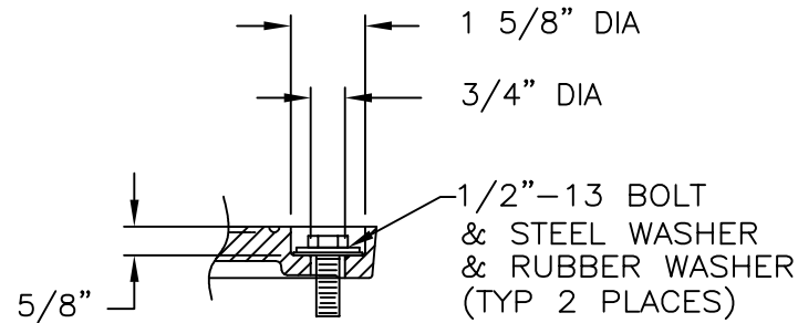
BOLTHOLE DETAIL
